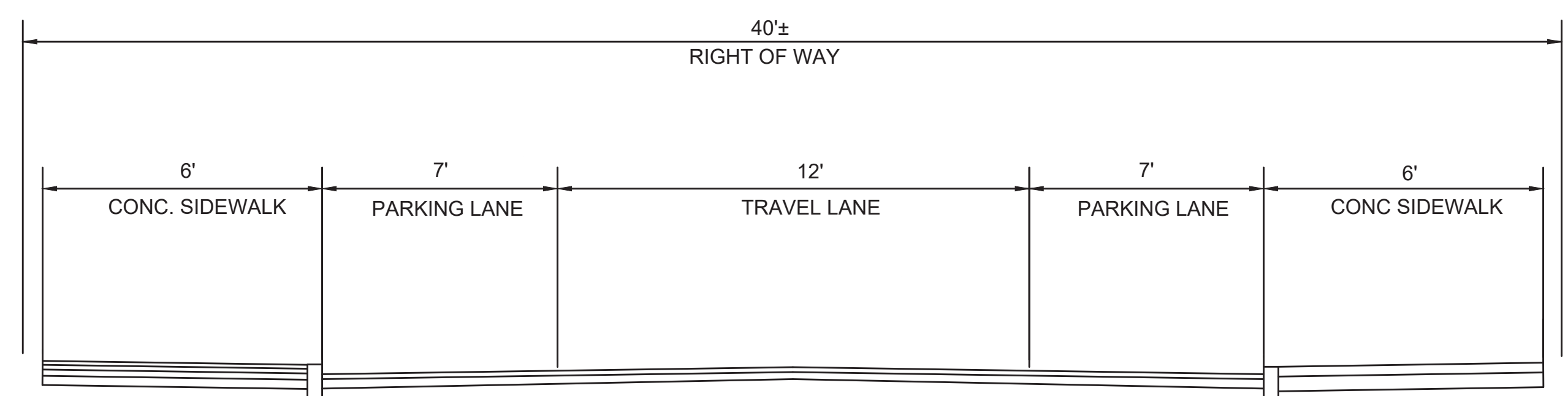
TYPICAL SECTION PLEASANT STREET TO SIDNEY STREET
