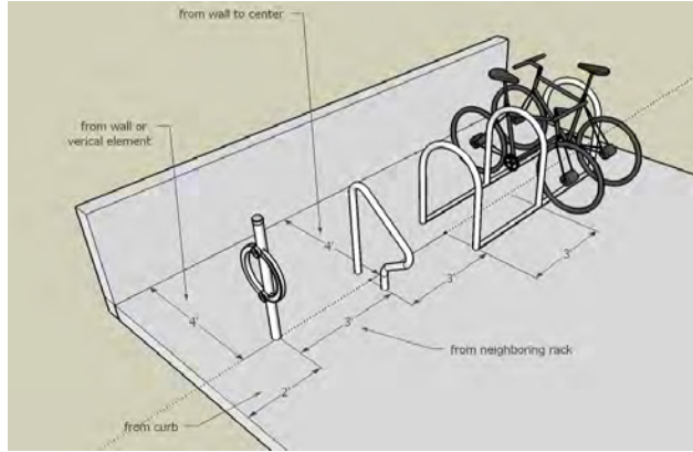
Bicycle Rack Types and Clearances
