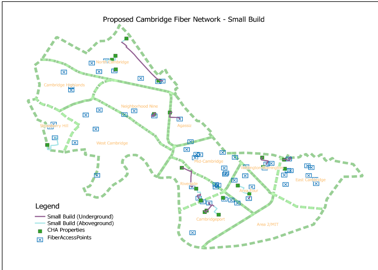
Figure 28: Small Network Buildout
