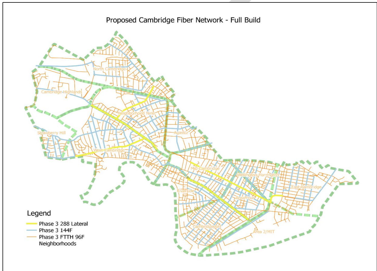
Figure 30: Large Network Buildout Map
