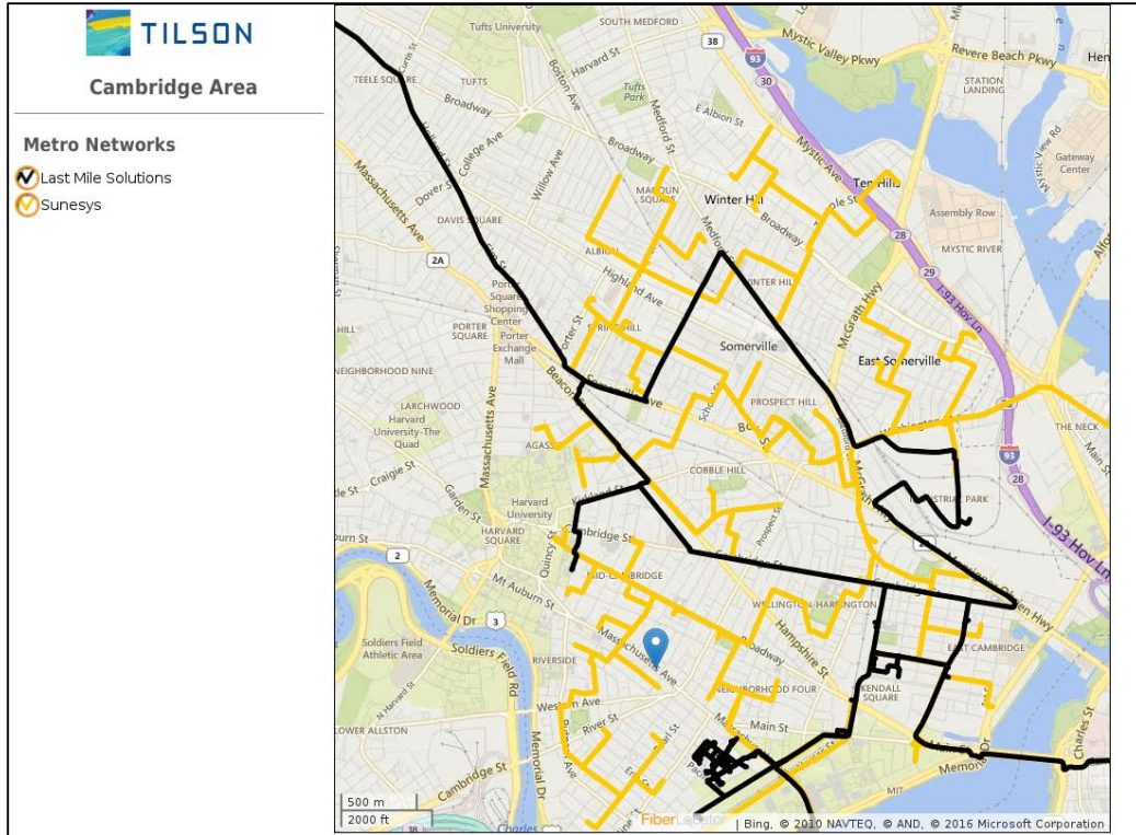
Figure 14: Map of Last Mile Solutions and Sunesys Dark Fiber
