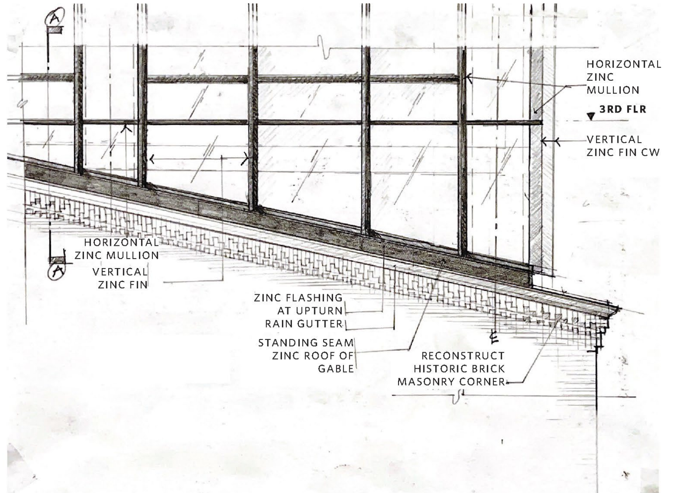
GABLE ROOF PARTIAL ELEVATION
