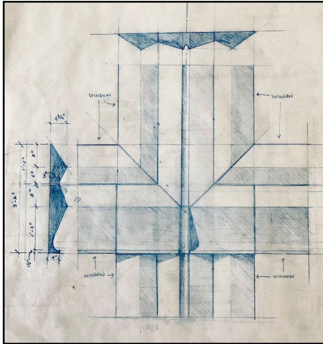
ELEVATION & SECTION SKETCH
