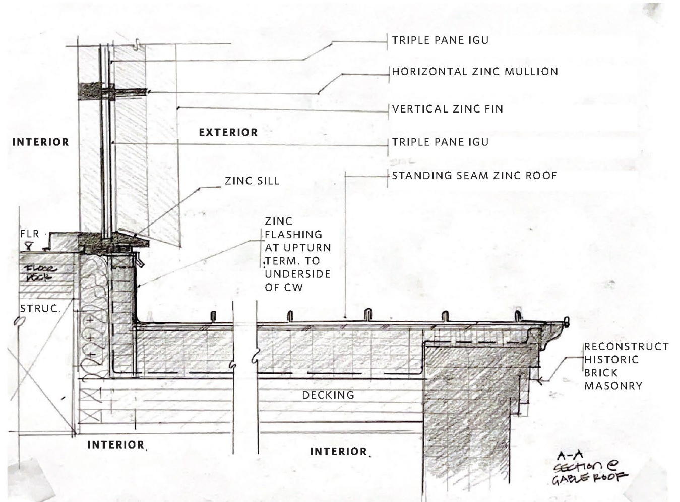
SECTION @ GABLE ROOF
