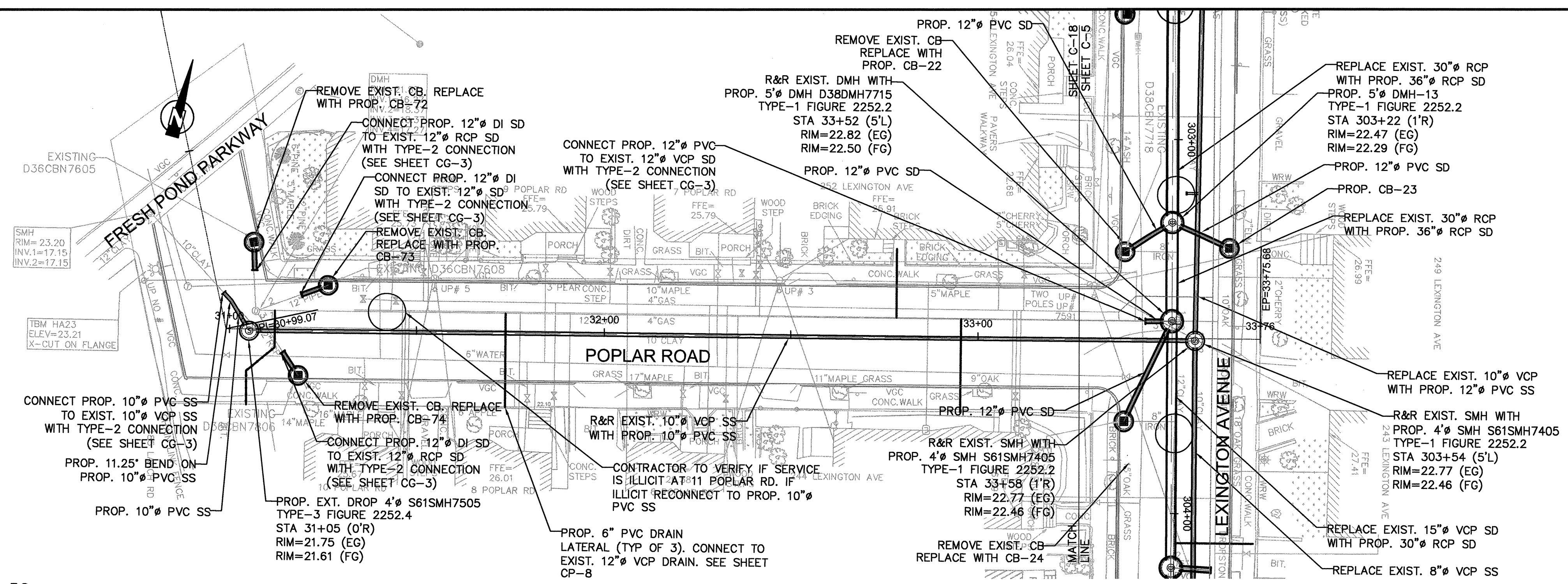
PLAN 1"=20'
