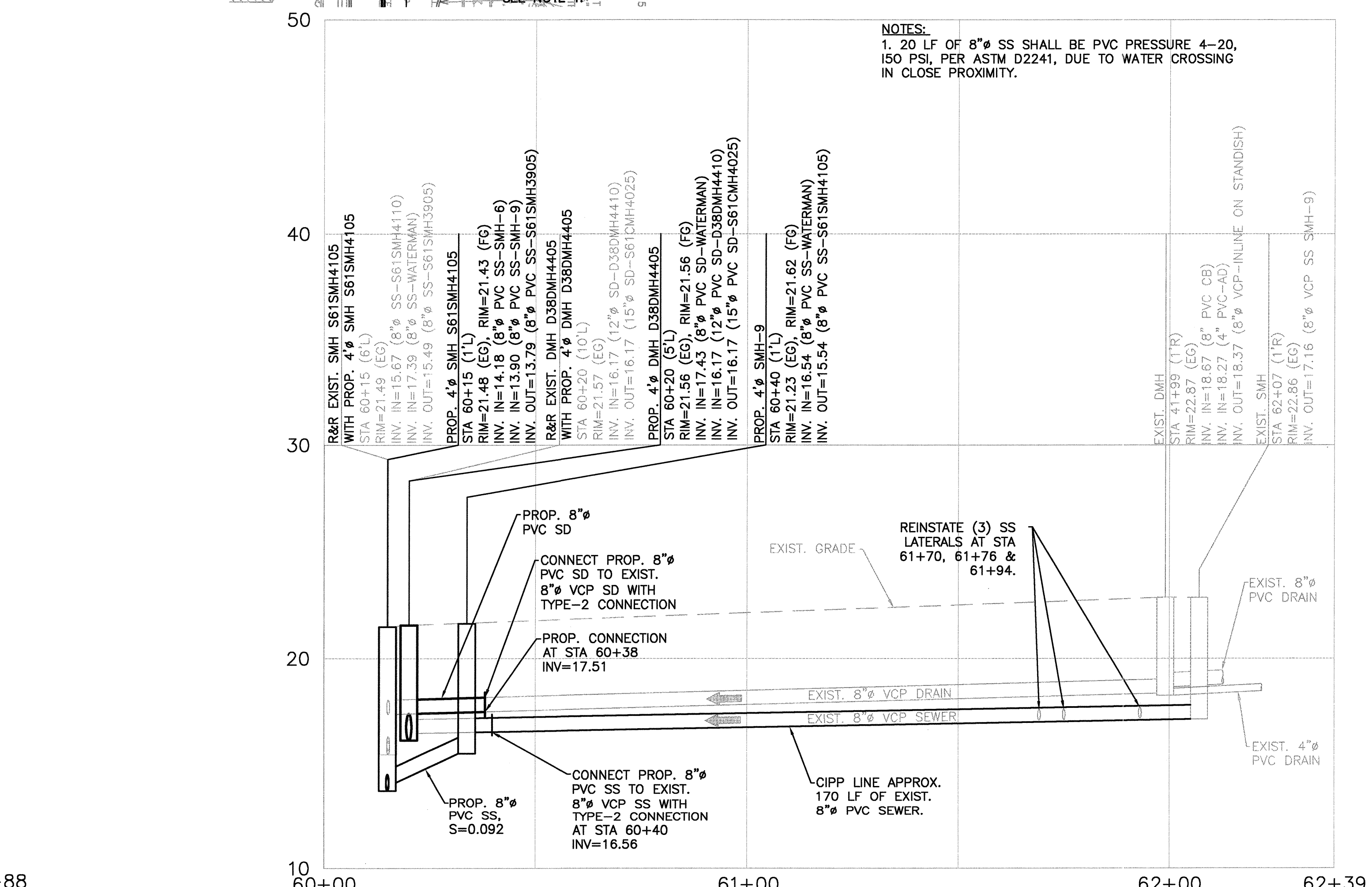
PROFILE HORIZONTAL SCALE: 1"=20' VERTICAL SCALE: 1"=4'
