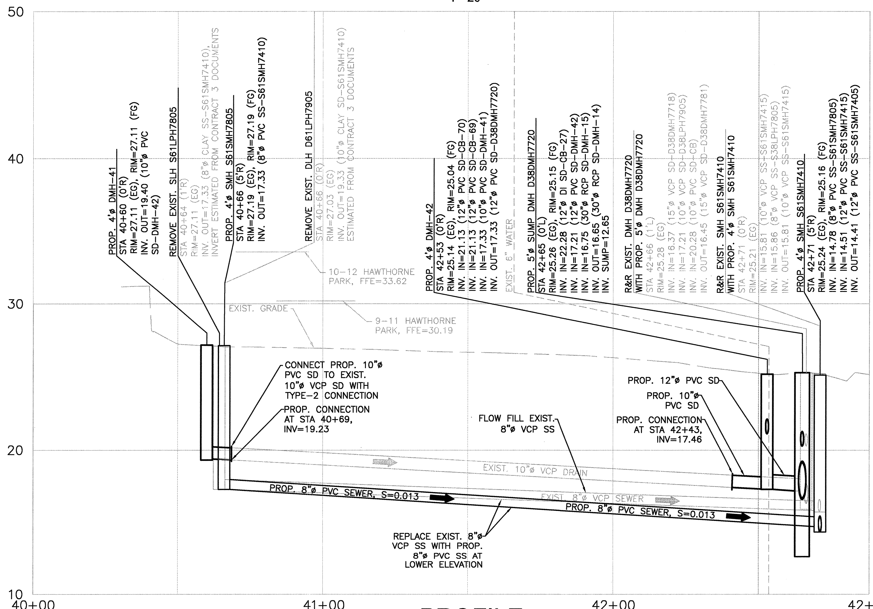
PROFILE HORIZONTAL SCALE: 1"=20' VERTICAL SCALE: 1"=4'
