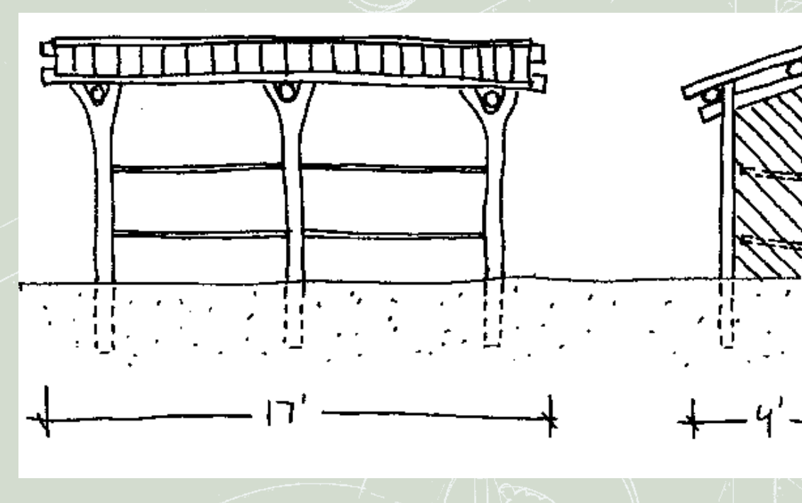
Block Storage Shed
