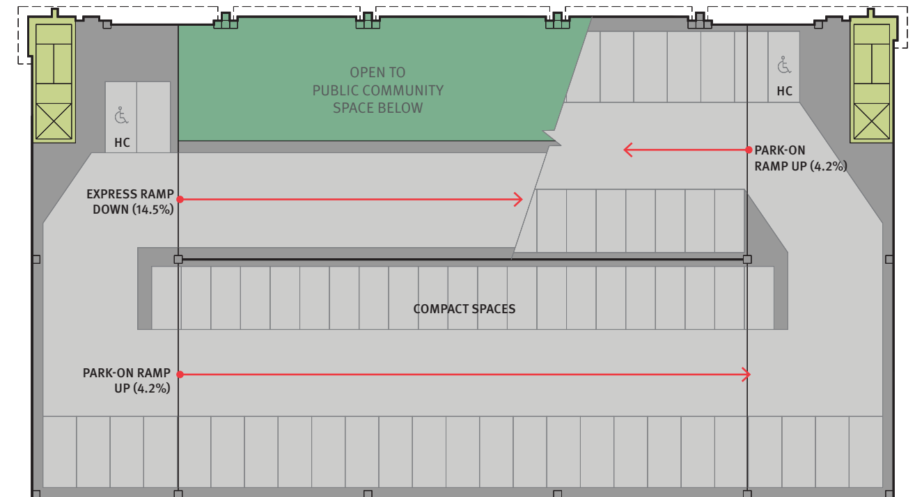
2ND FLOOR //
