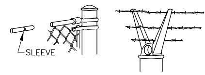
ONE-PIECE (6-WIRE)
