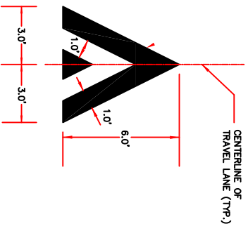
"FIELD" PAVEMENT SETTING DETAIL
