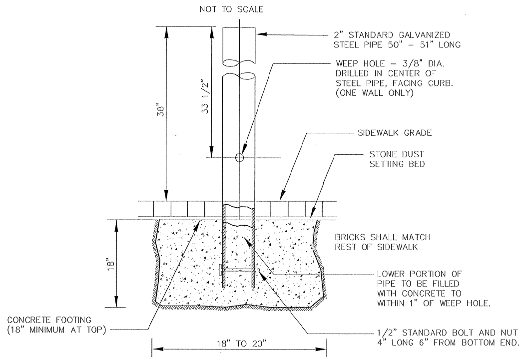
PARKING METER POST ON BRICK SIDEWALK
