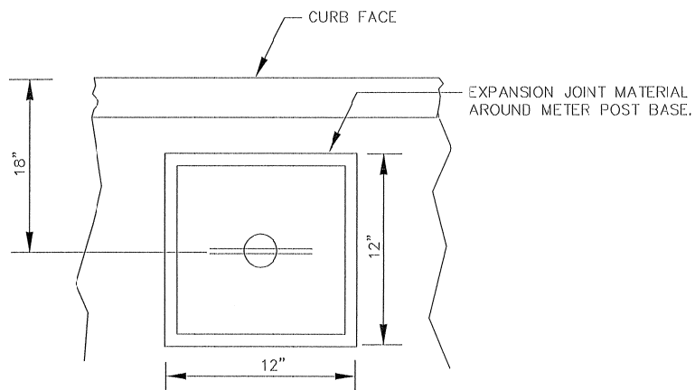
PLAN - PARKING METER POST
