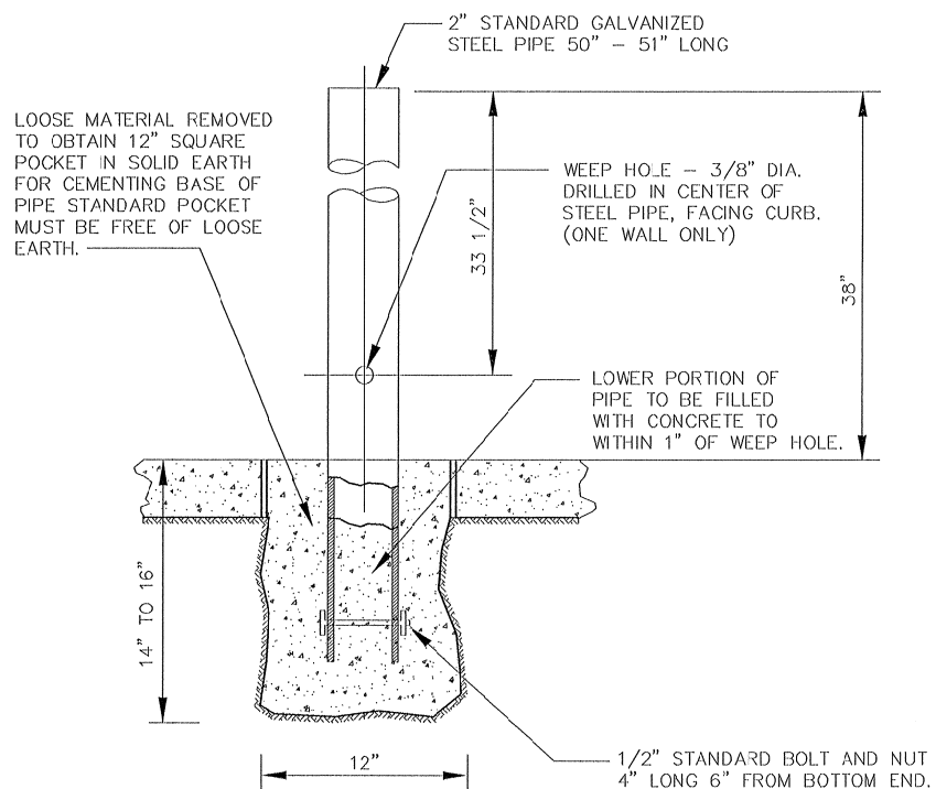
PARKING METER POST ON CONCRETE SIDEWALK
