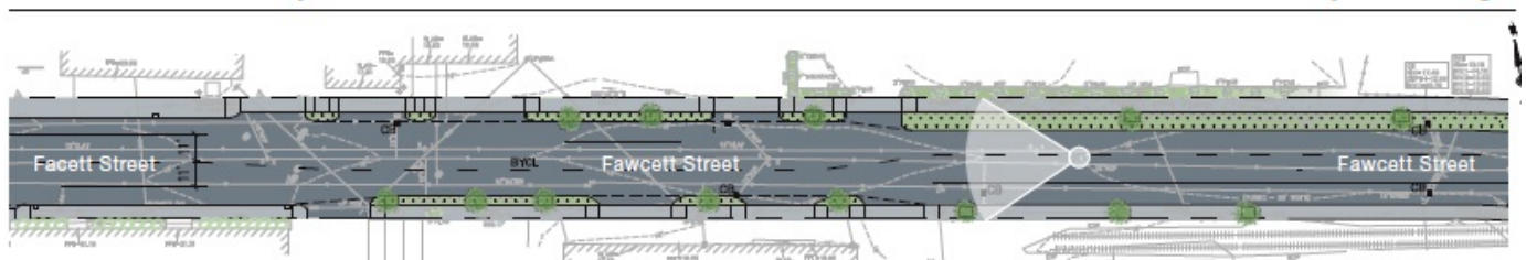
Fawcett Street Improvements Concord Avenue to Smith Place
