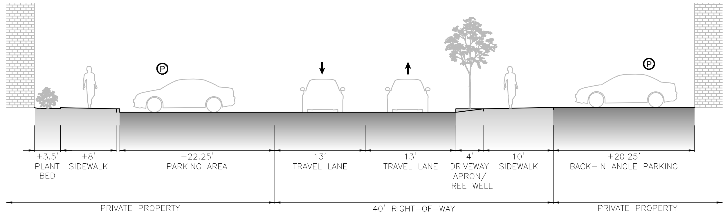
TYPICAL SECTION C - RUFO ROAD
