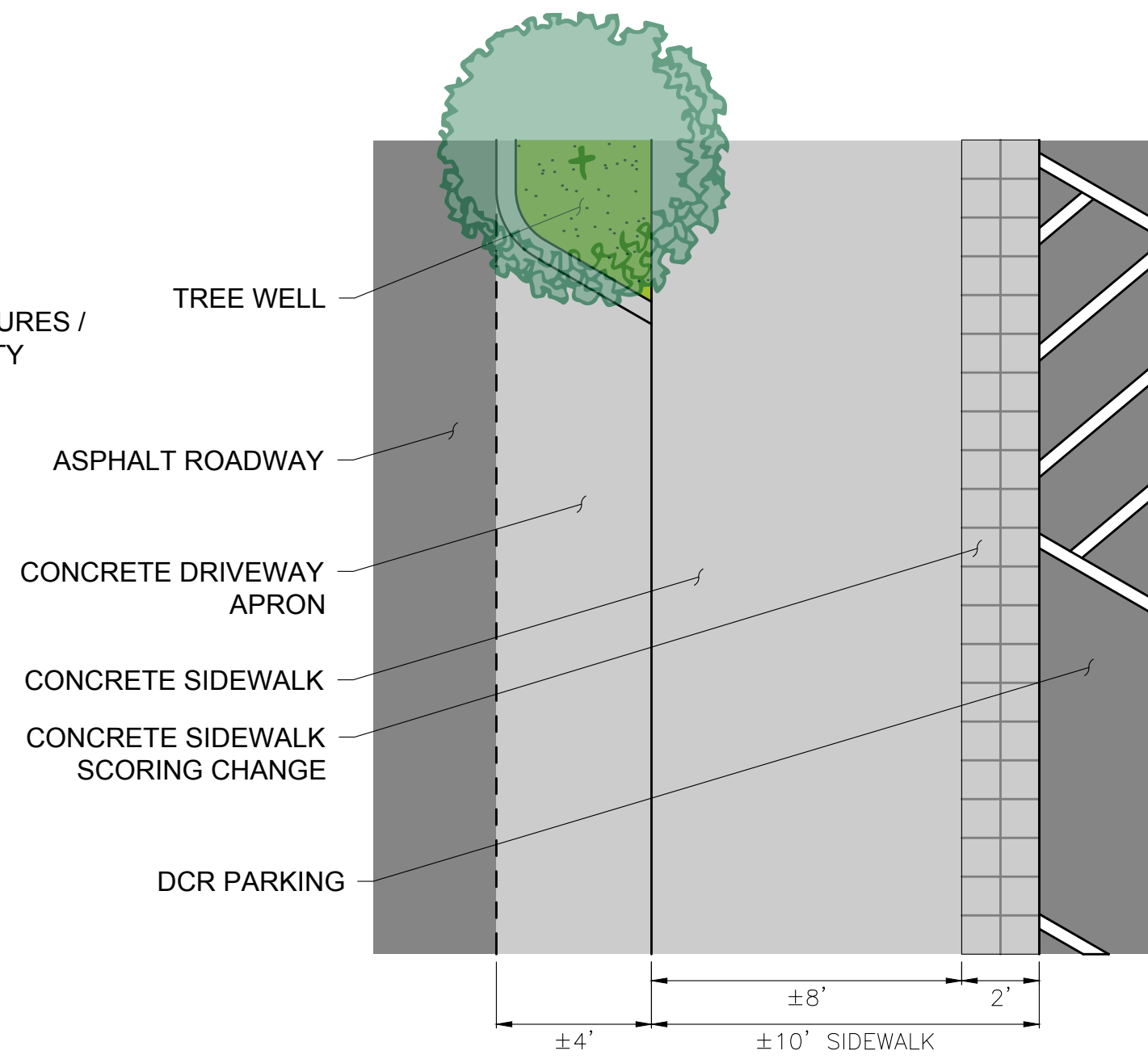
TYPICAL RUFO ROAD SIDEWALK
