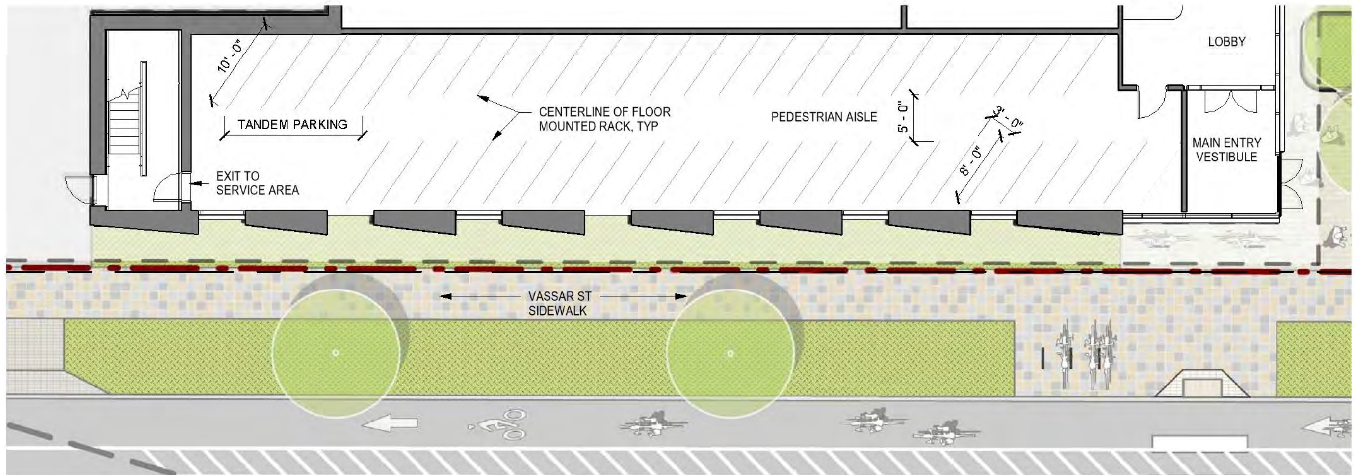
LONG TERM BICYCLE PARKING - LEVEL 1
