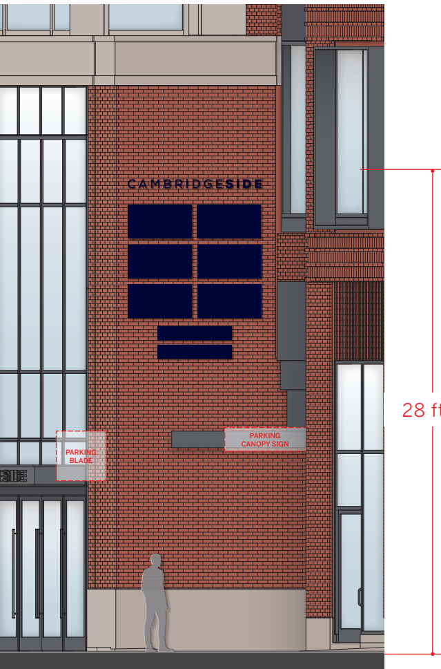
MOUNTING ELEVATION 100 CAMBRIDGESIDE (EAST) SCALE 1/8" = 1'-0"
