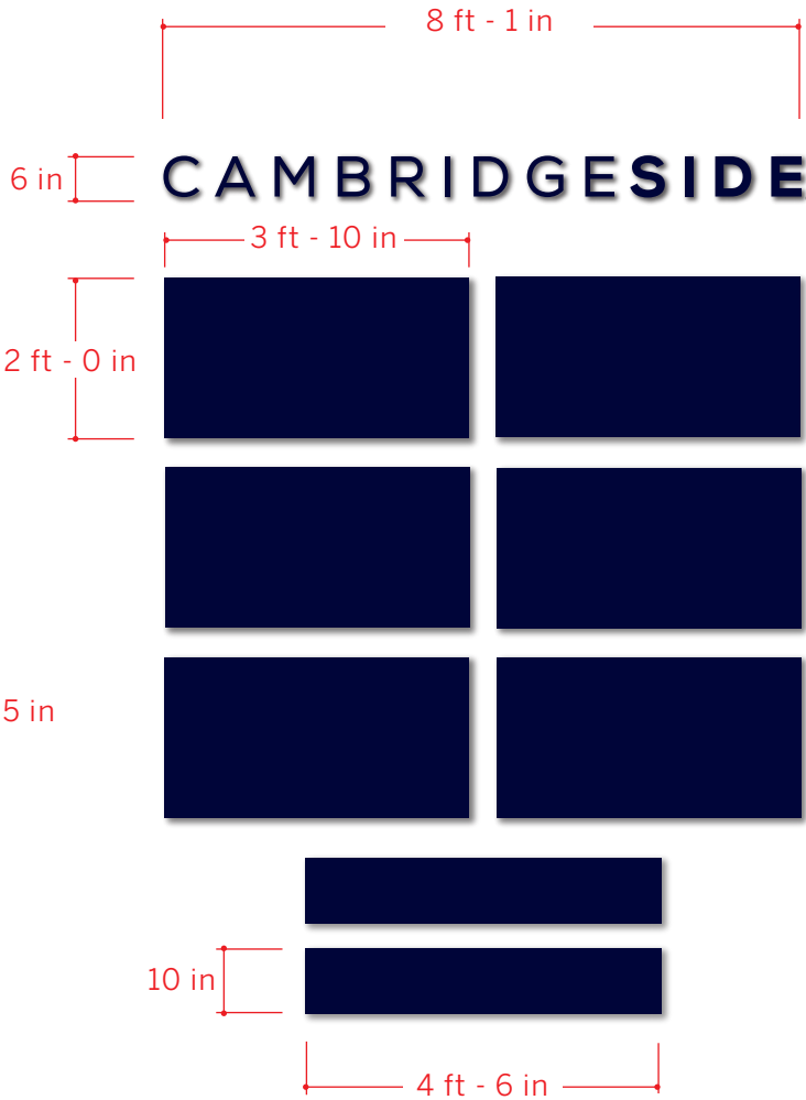
EXAMPLE CONFIG. #1 SCALE 3/8" = 1'-0"
