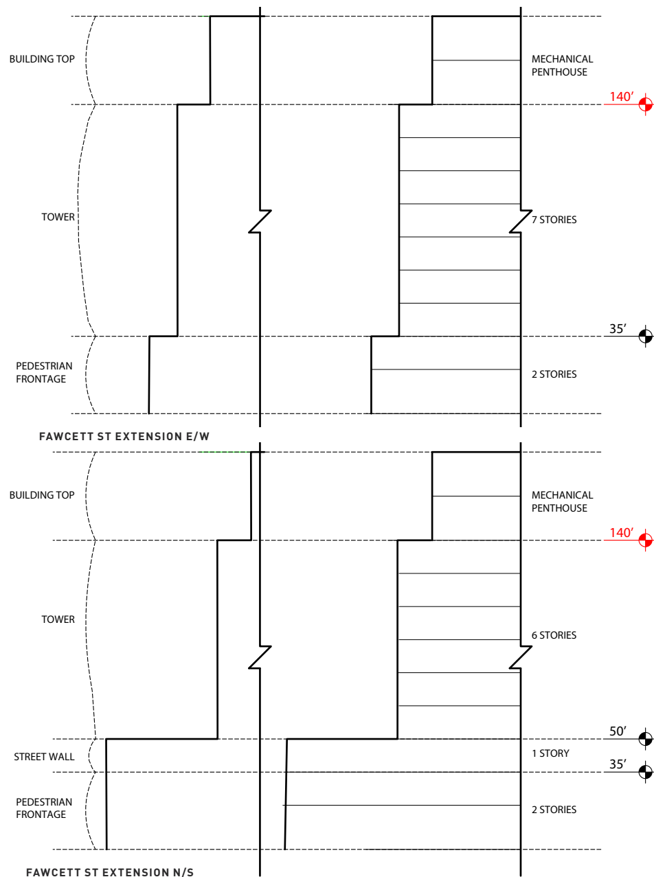
Figure 1L.13b: Block Guidelines - C6 Healthpeak PUD Master Plan | Cambridge, MA
