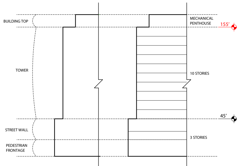
Figure 1L.20b: Block Guidelines - R4
