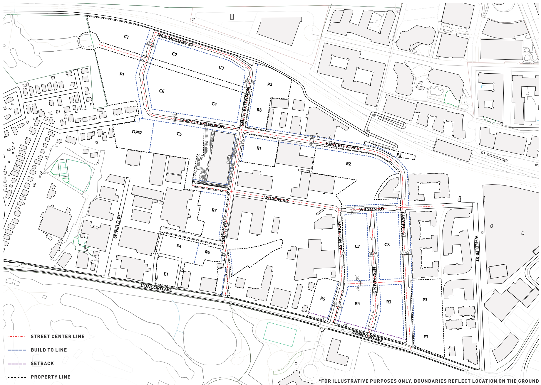
Figure 1L.5: Site Development Plan - Build to Line
