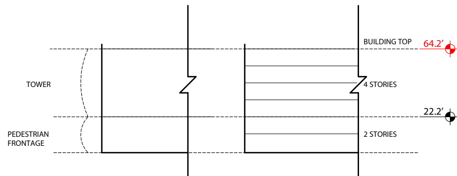
Figure 1L.18b: Block Guidelines - P3 Healthpeak PUD Master Plan | Cambridge, MA
