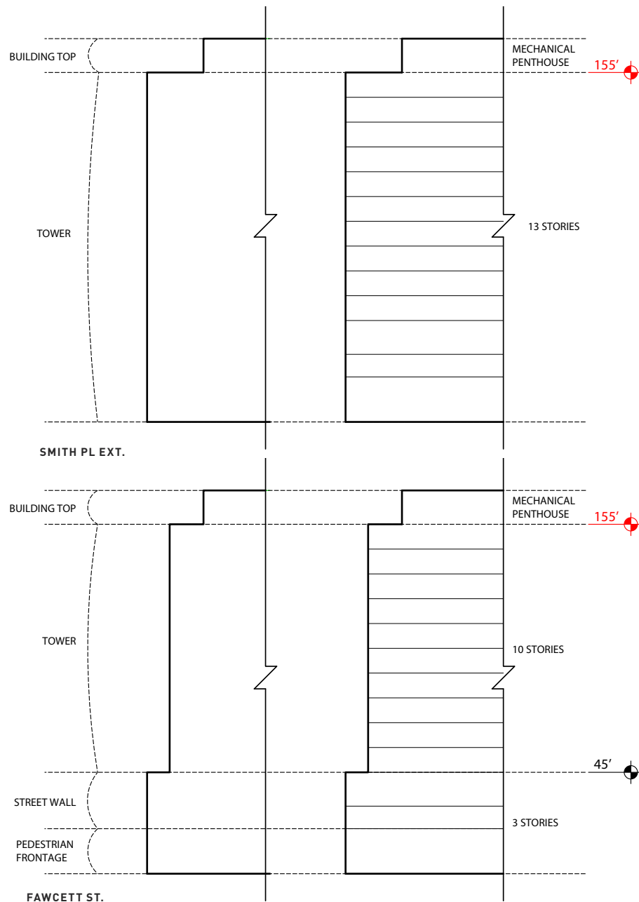
Figure 1L.25b: Block Guidelines - R8
