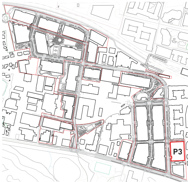
Figure 1L.18a: Block Guidelines - P3
