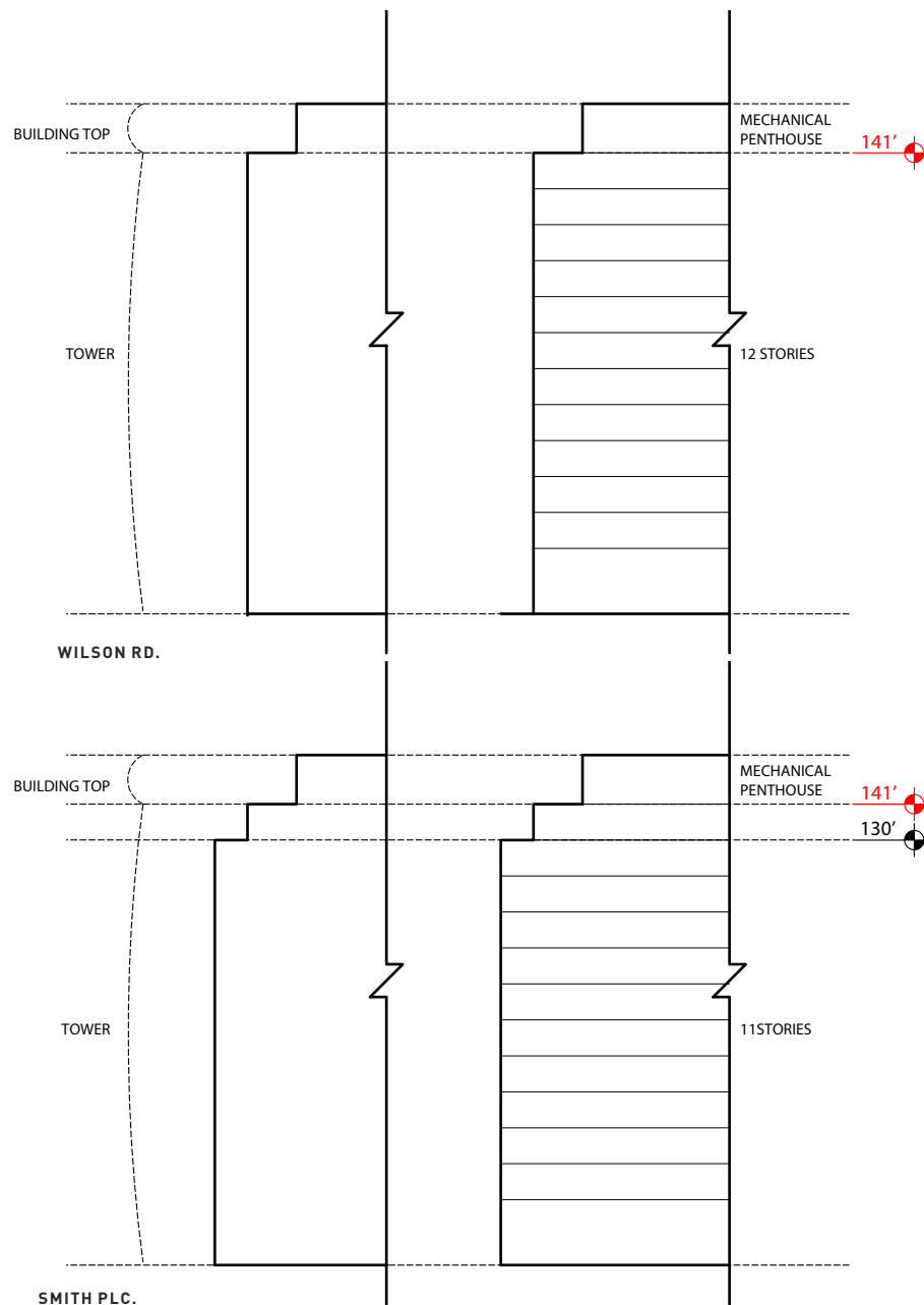
Figure 1L.24b: Block Guidelines - R7
