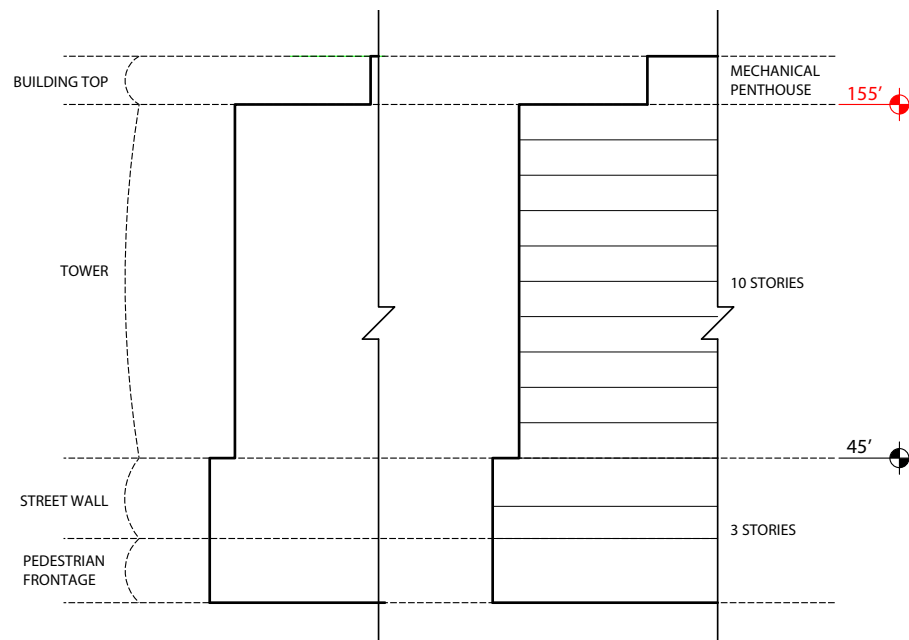
Figure 1L.15b: Block Guidelines - R2 Healthpeak PUD Master Plan | Cambridge, MA
