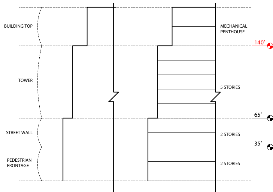
Figure 1L.9b: Block Guidelines - C3 Healthpeak PUD Master Plan | Cambridge, MA
