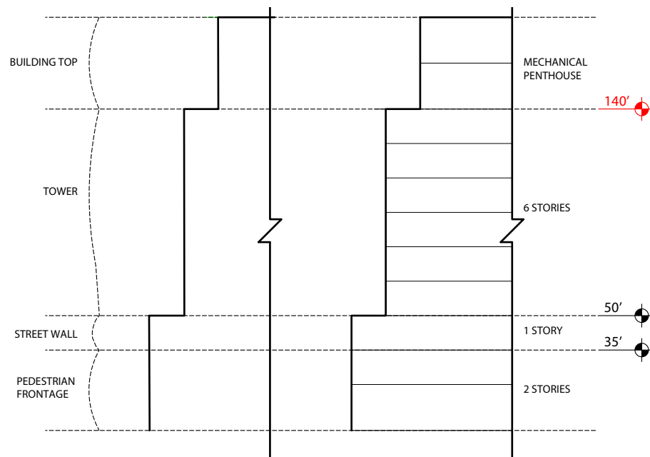
Figure 1L.7b: Block Guidelines - C1 Healthpeak PUD Master Plan | Cambridge, MA
