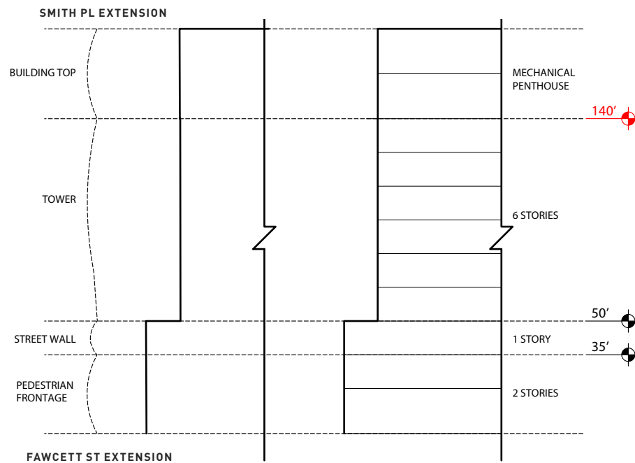
Figure 1L.11b: Block Guidelines - C4 Healthpeak PUD Master Plan | Cambridge, MA
