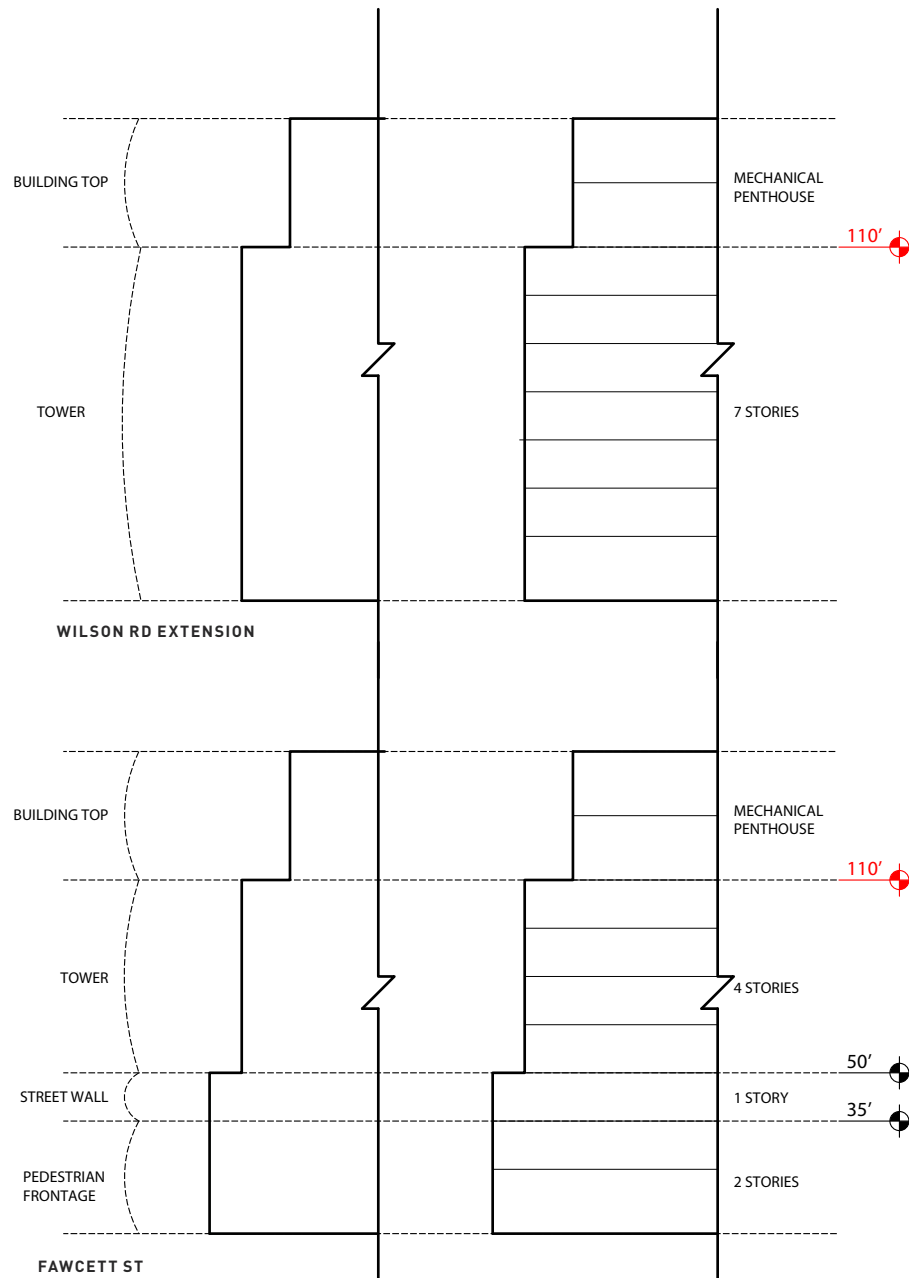
Figure 1L.17b: Block Guidelines - C8
