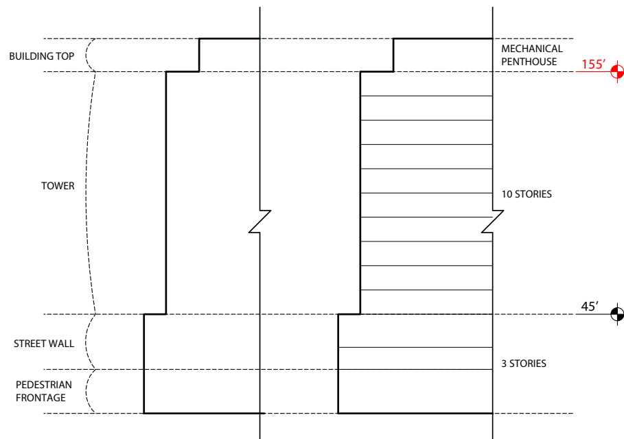
Figure 1L.19b: Block Guidelines - R3 Healthpeak PUD Master Plan | Cambridge, MA
