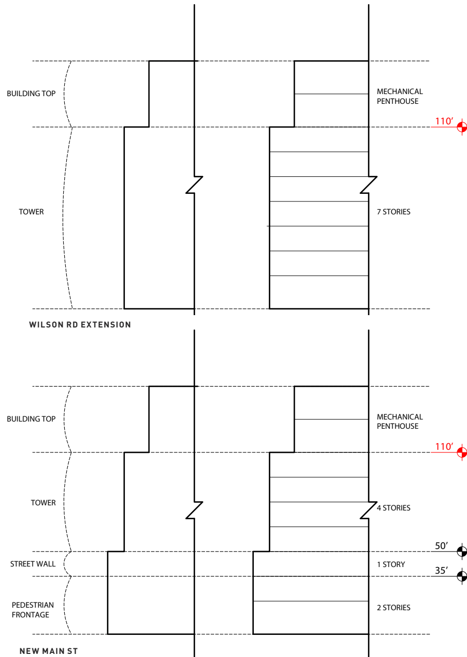
Figure 1L.16b: Block Guidelines - C7
