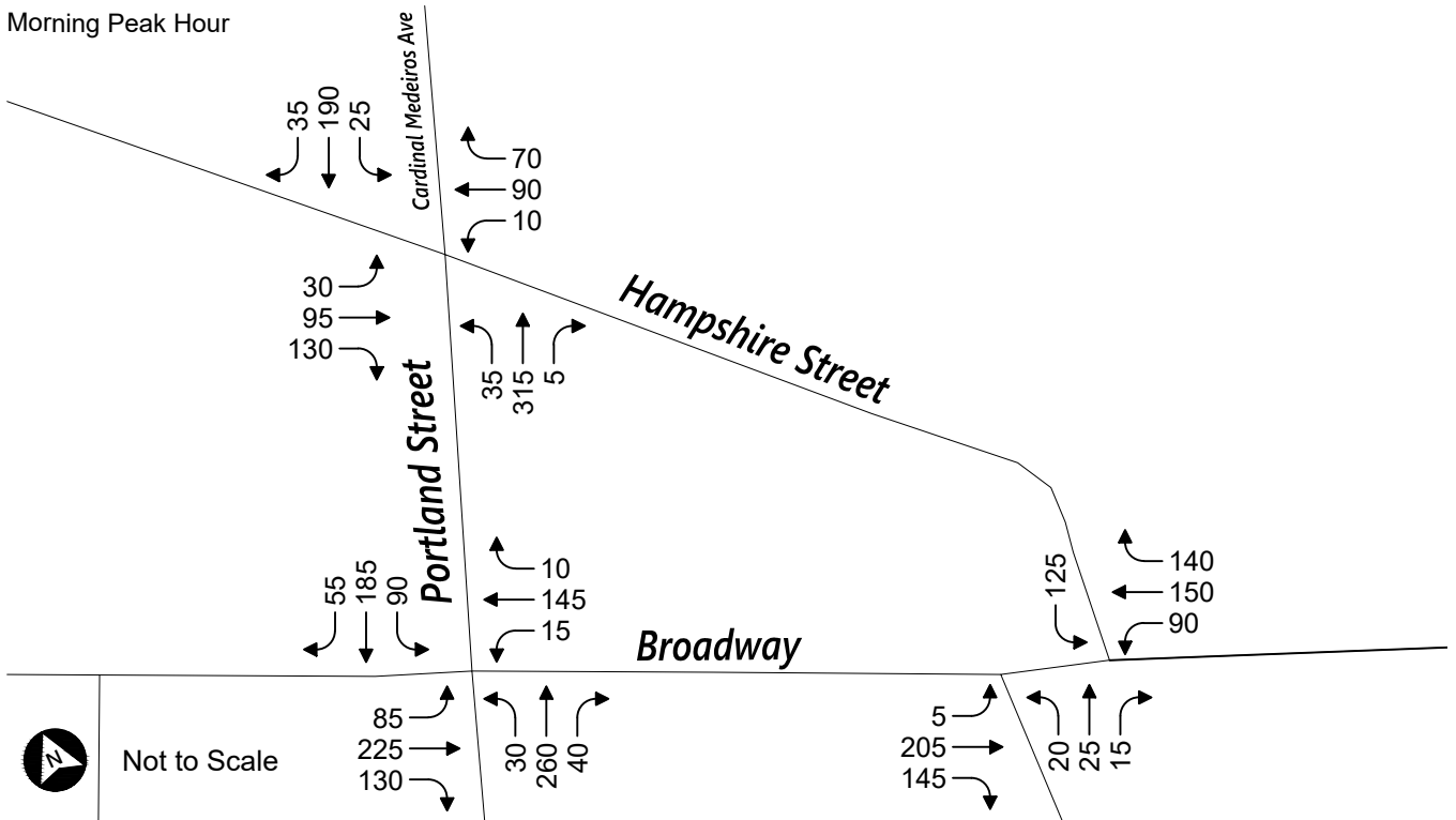
Figure 5: Proposed Peak Hour Vehicle Volumes
