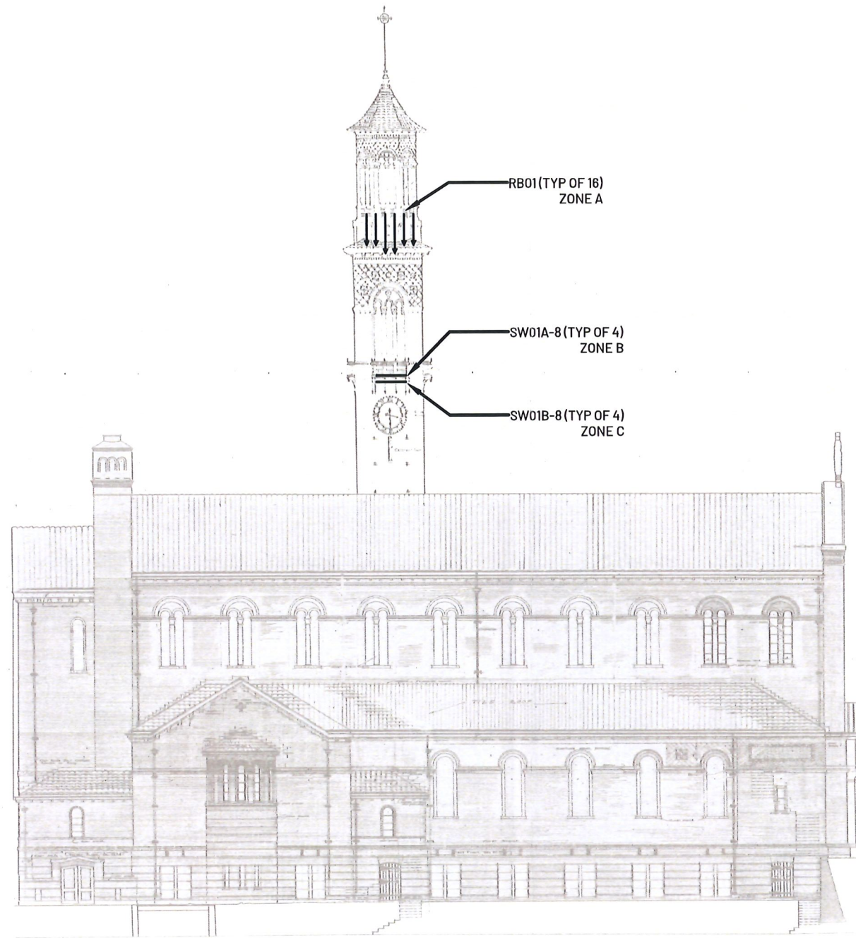
1 EAST ELEVATION R2.05 SCALE: 1/16"=1'-0"
