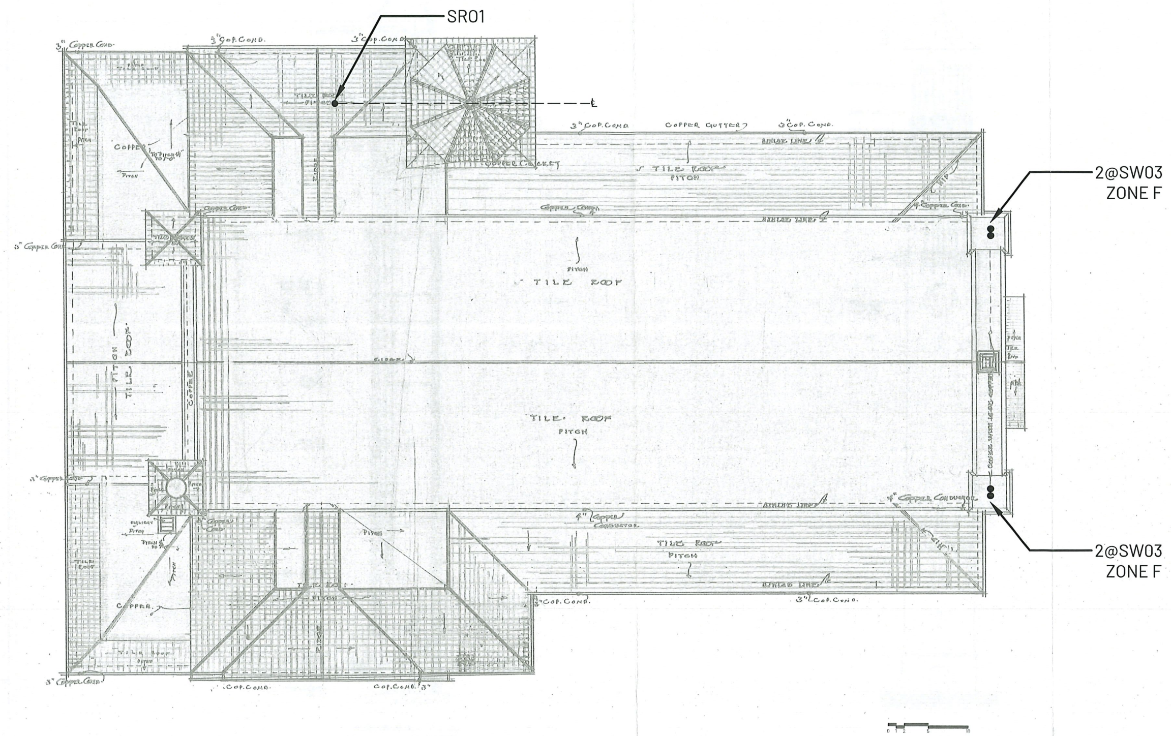
1 R2.12 ROOF PLAN SCALE: 3/16"=1'-0"
