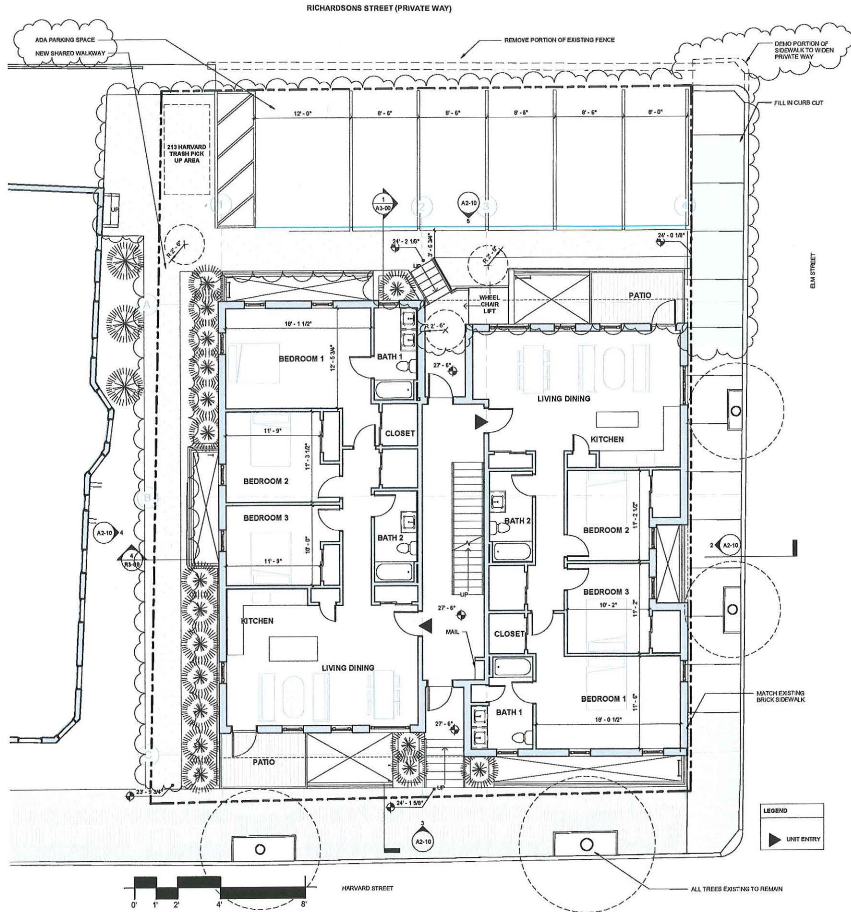
① LEVEL 1 FLOOR PLAN 3/16" = 1'-0"
