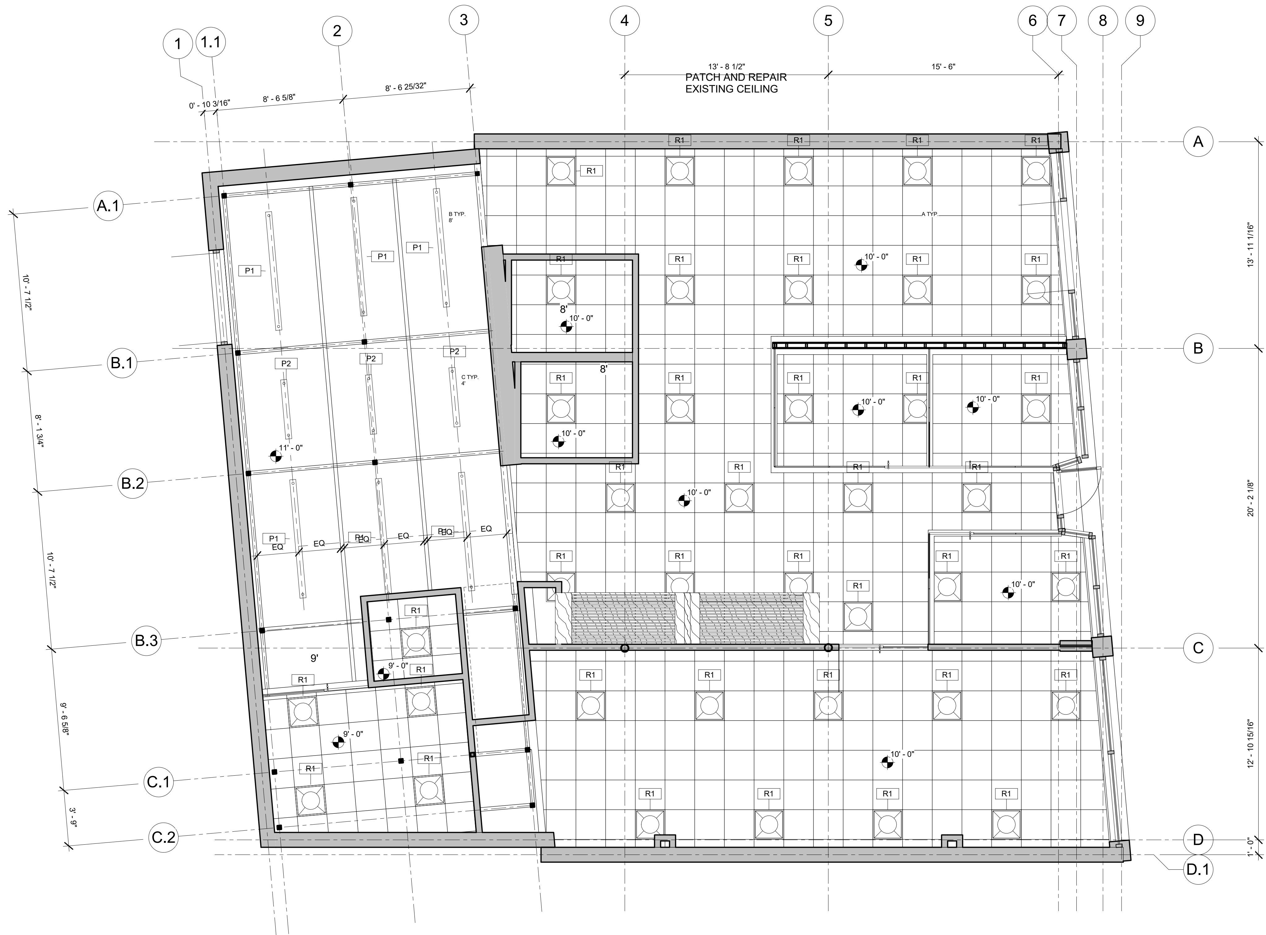
1 LEVEL 1 RCP 1/4" = 1'-0"
