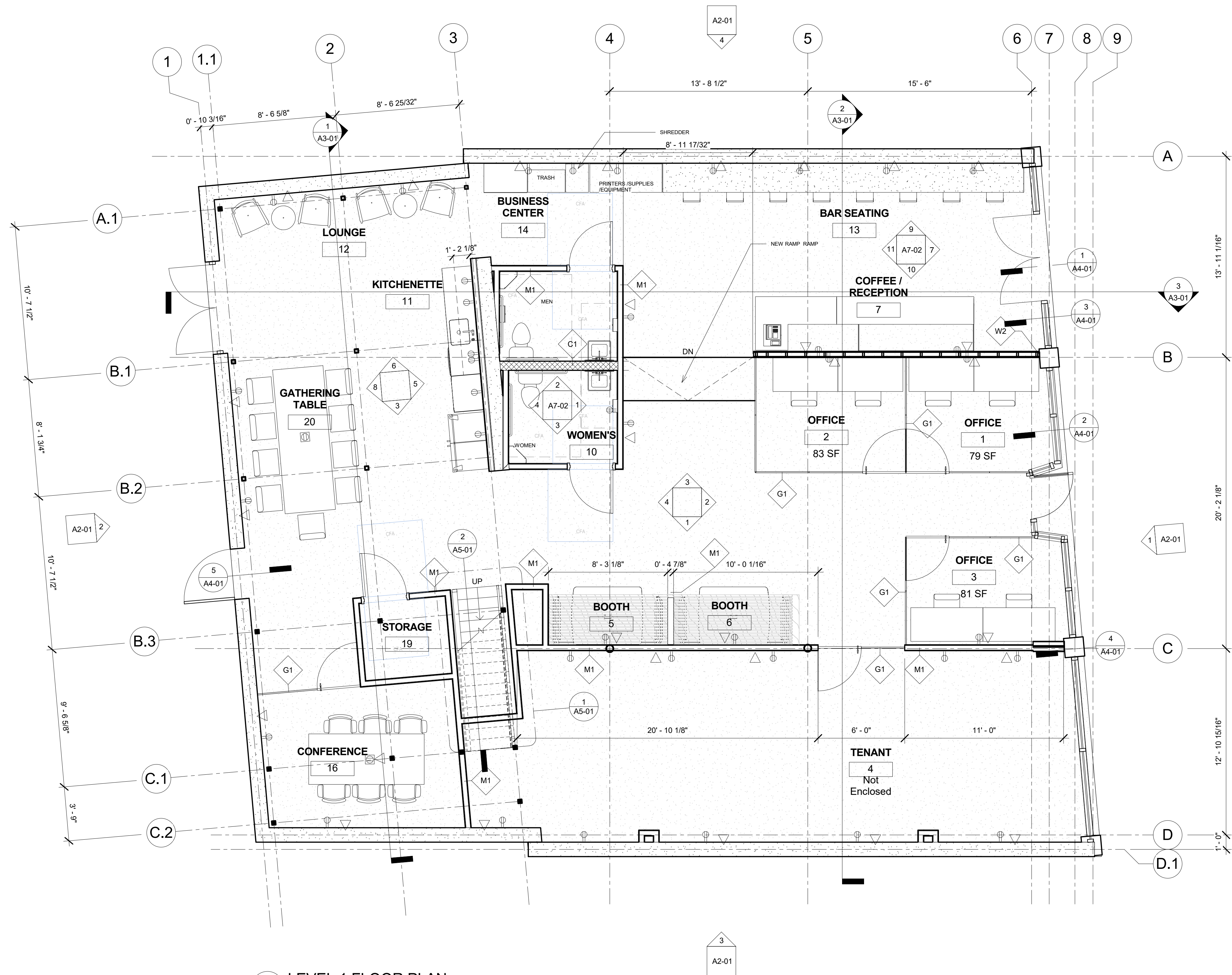
1 LEVEL 1 FLOOR PLAN 1/4" = 1'-0"
