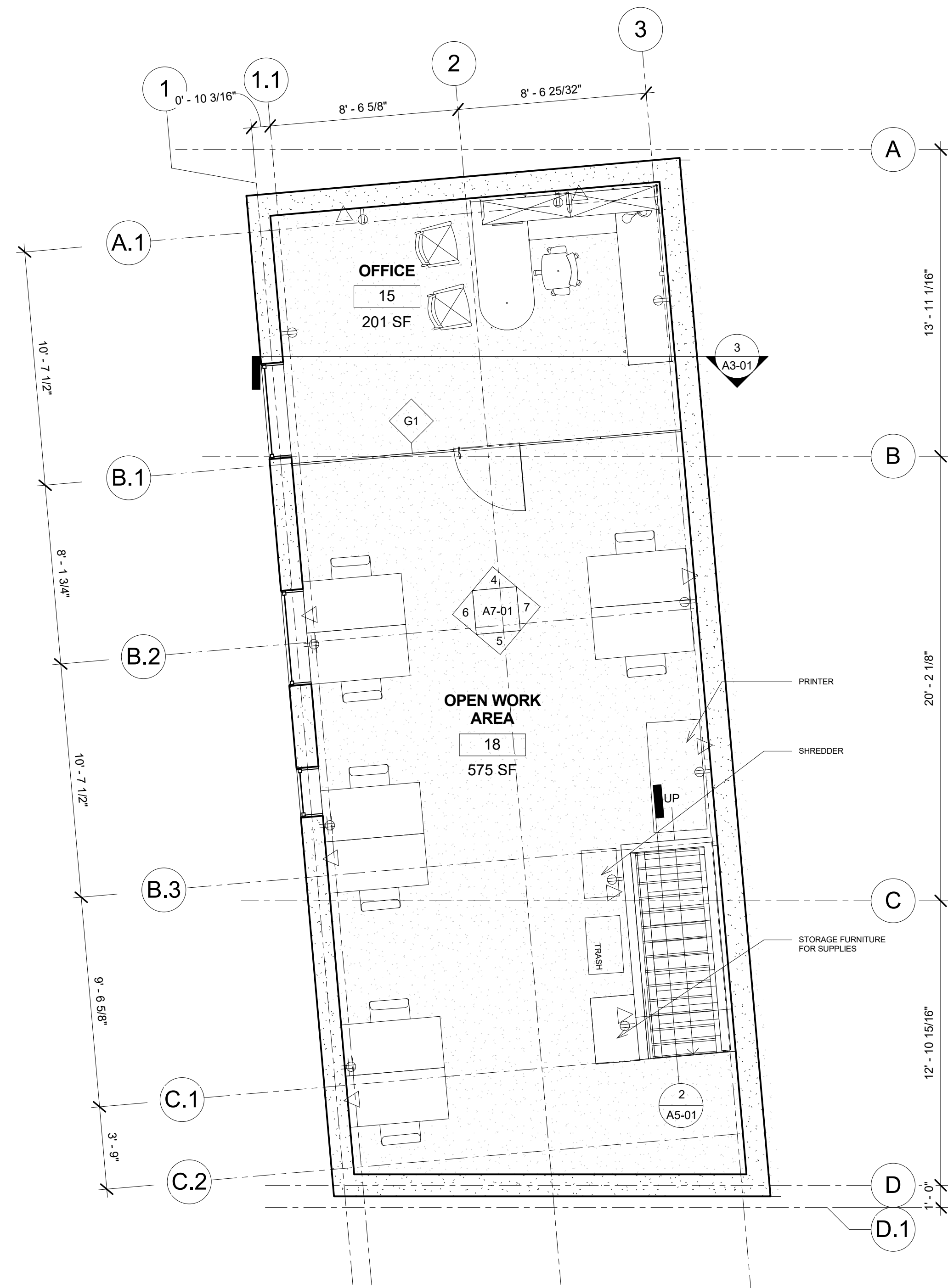
1 LEVEL 2 FLOOR PLAN 1/4" = 1'-0"
