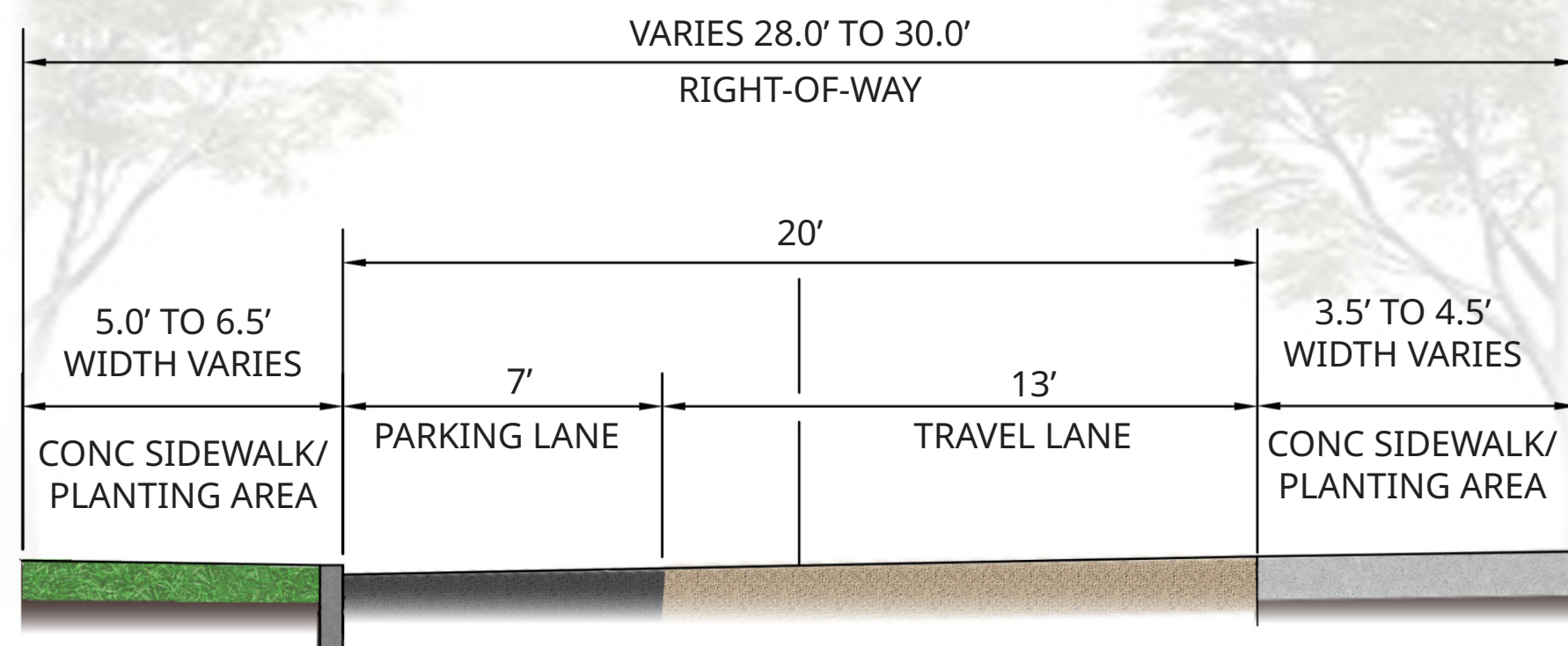
TYP. SECTION CUT A-A KIRKLAND ROAD
