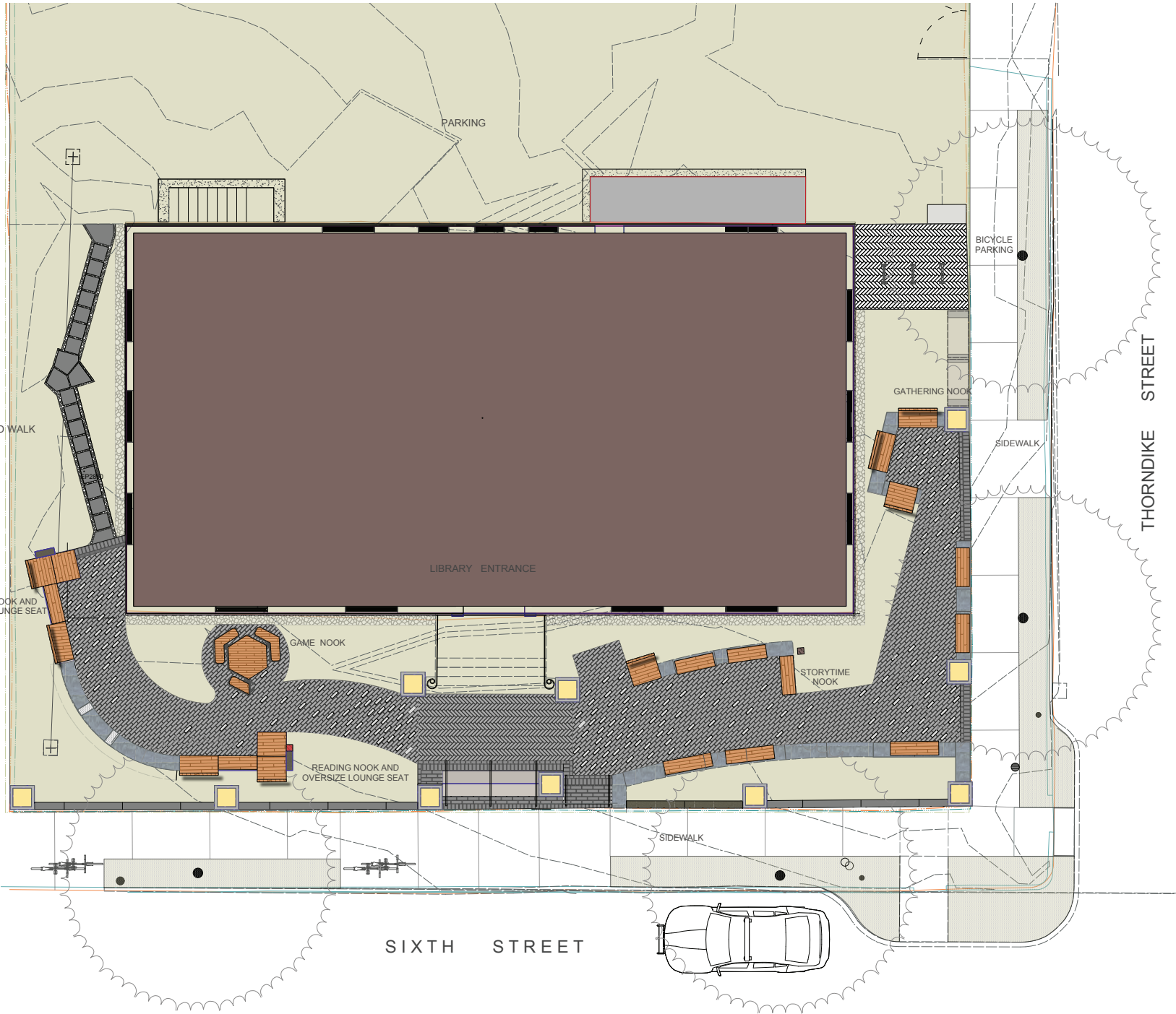
HARDSCAPE AND SITE FURNISHING PLAN
