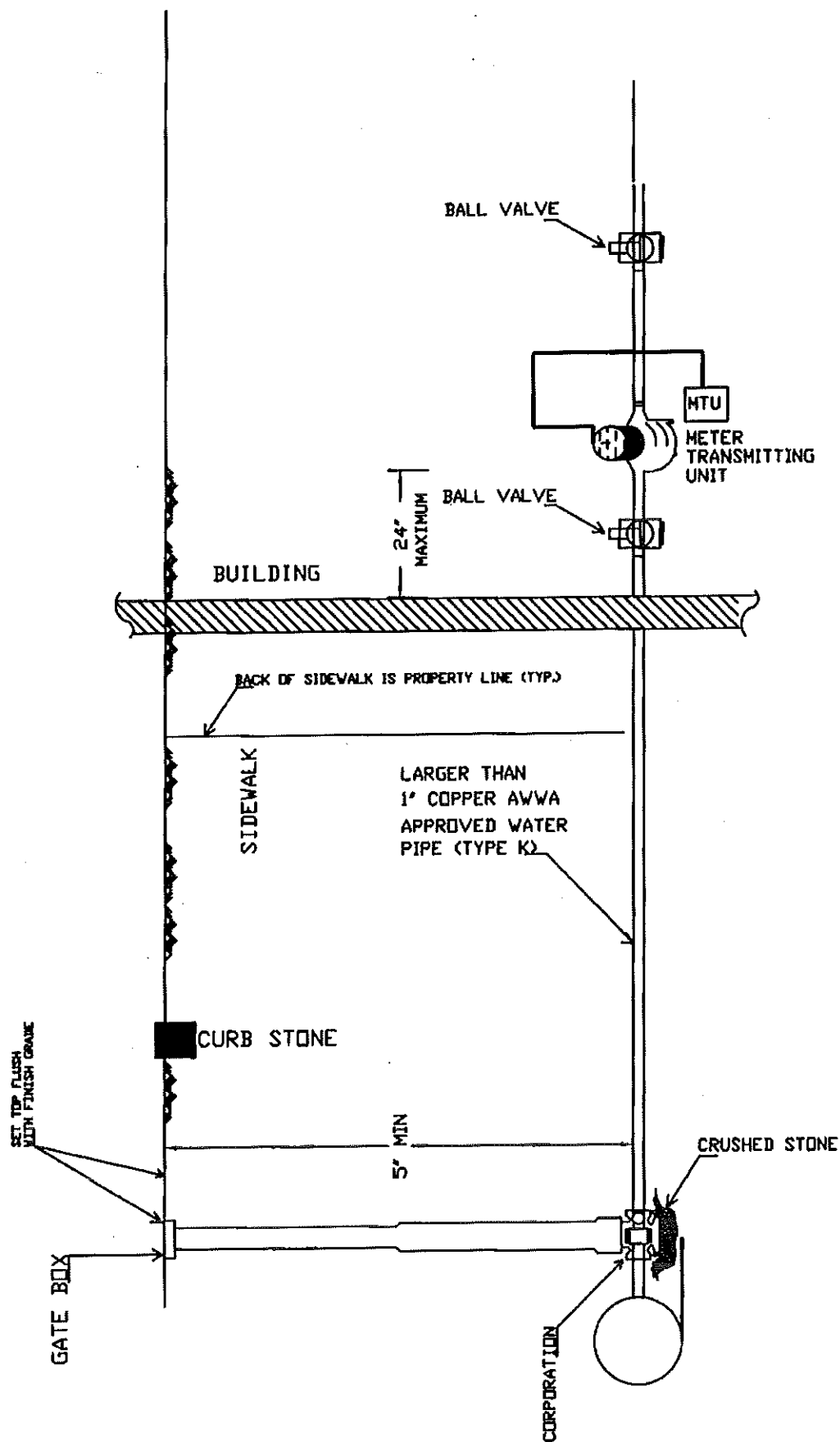
TYPICAL LARGER THAN 1" SERVICE & METER INSTALLATION
