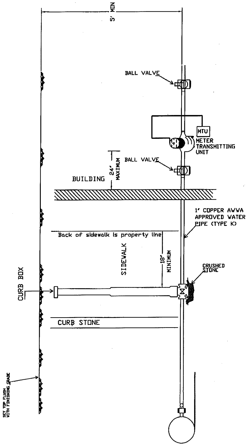
TYPICAL 1" SERVICE & METER INSTALLATION NOT TO SCALE
