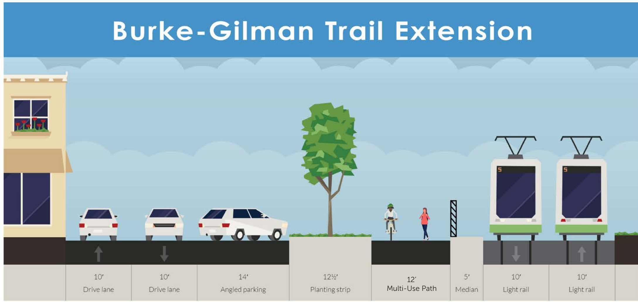
Typical cross-section of Burke-Gilman Trail
