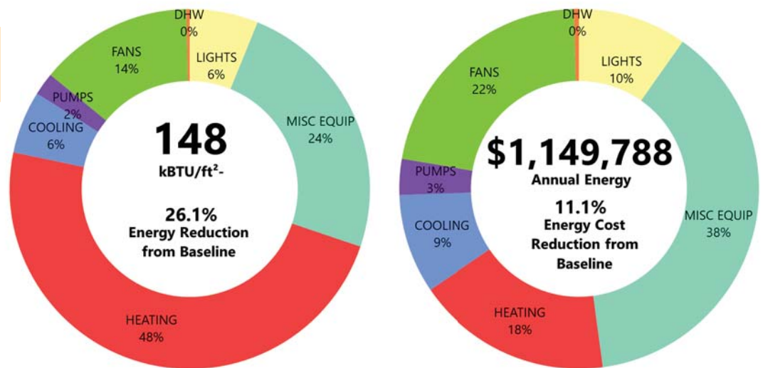
DESIGN MODEL ENERGY / COST BY END USE
