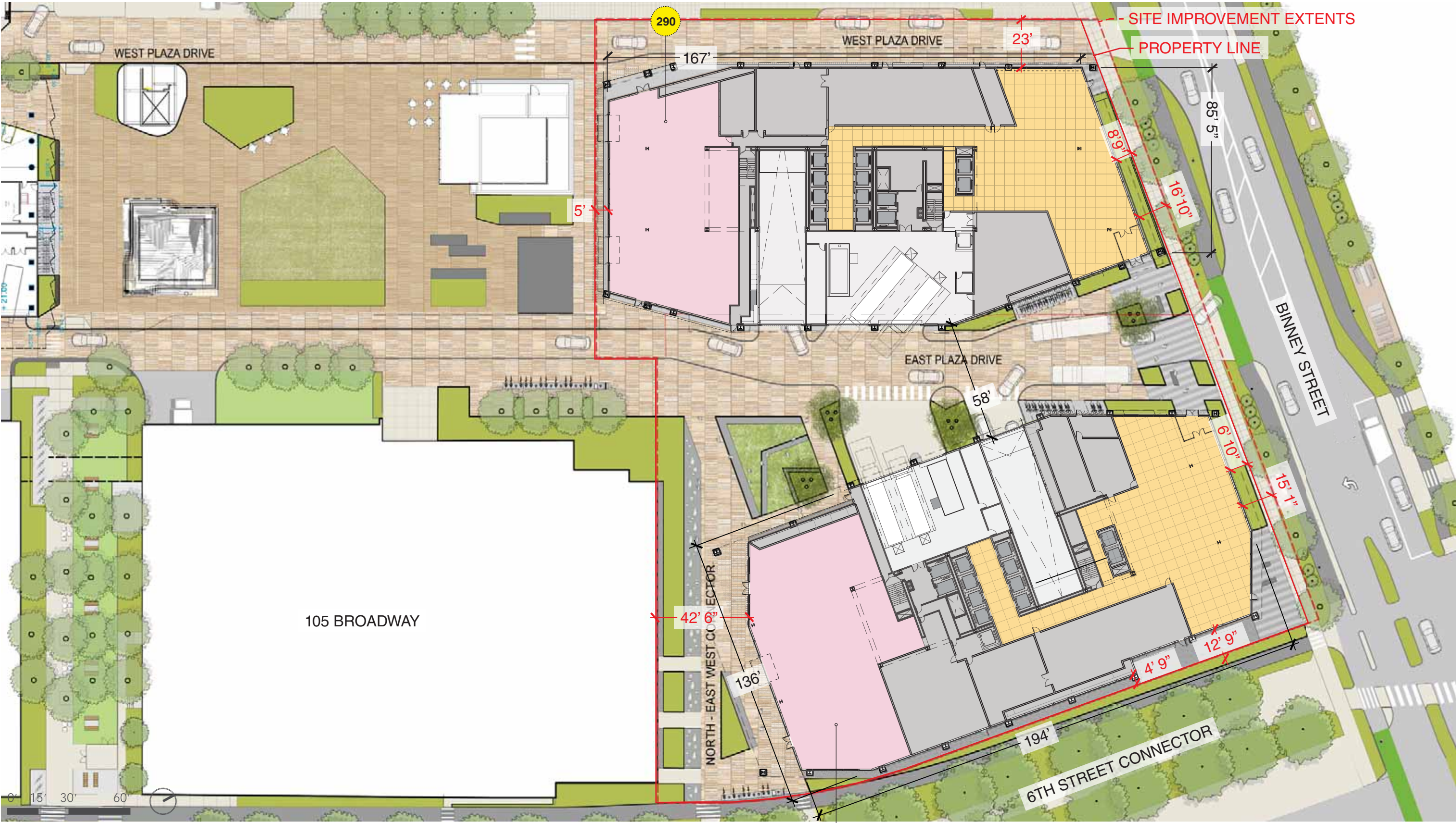
290 BINNEY STREET THIS COMMUNICATES THE DESIGN INTENT OF BOTH COMMERCIAL BUILDINGS
