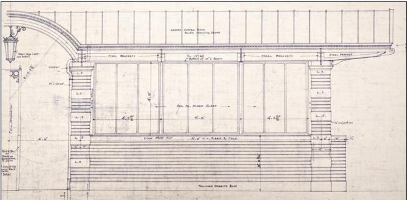
East Elevation, north side. Construction drawing, 1927 BERY Collection, CHC
