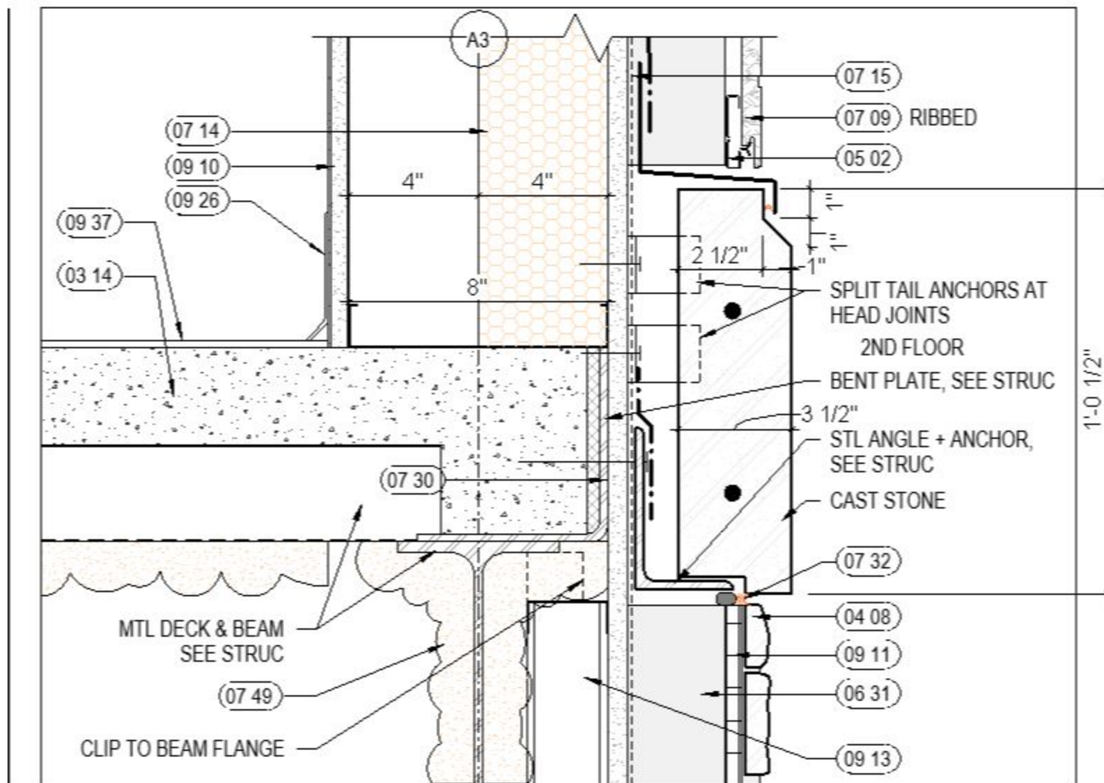
3 VENEER STONE TO SIDING TRANSITION DTL 3" = 1'-0"
