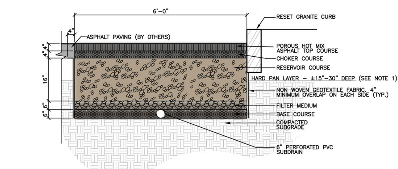
TYPICAL SECTION - POROUS PAVEMENT
