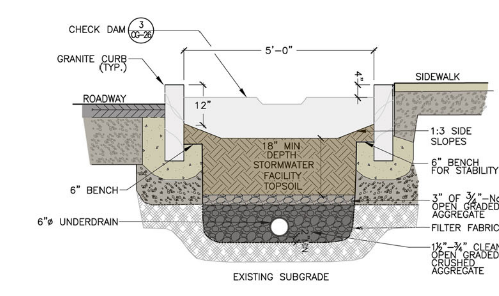
TYPICAL SECTION - BIOBASIN TYPE II
