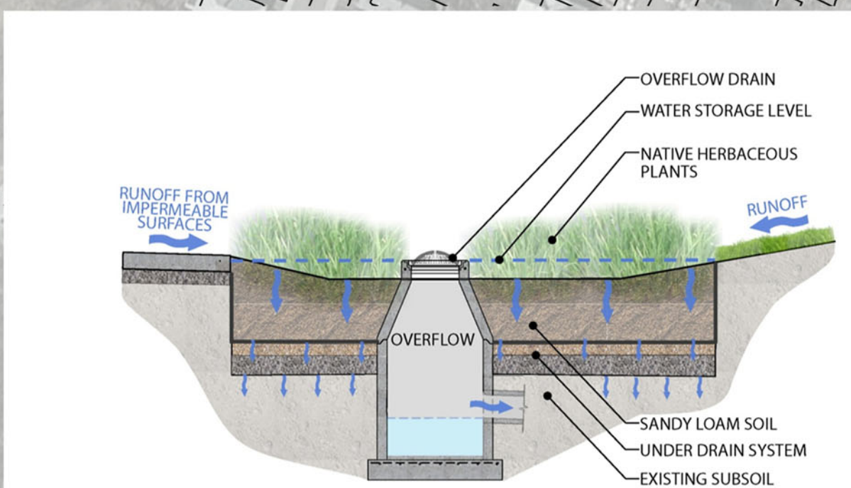
TYPICAL SECTION - BIOBASIN TYPE I
